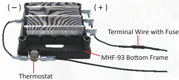
Example 1 – Standard Single Insulation Wiring – Part Number: MH-2130S-93 S 4
