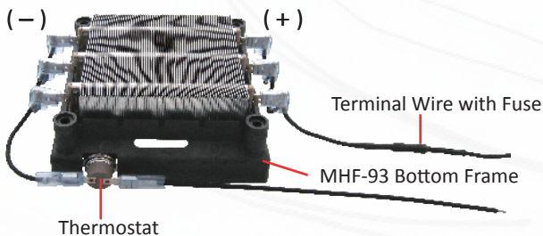
Example 2 – Standard Double Insulation Wiring – Part Number: MH-2120S-93 D 4
